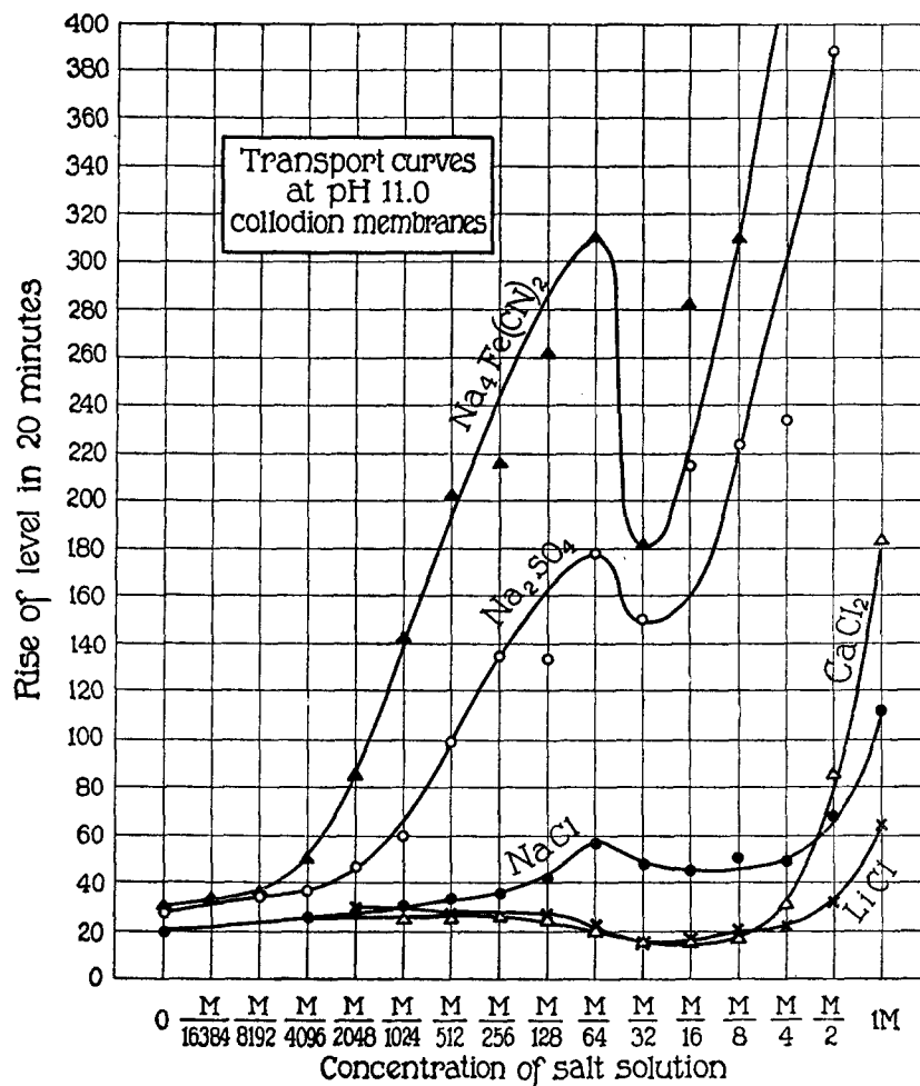
FIG. 3. Transport curves at pH 11.0. The electrical effect is visible only for \text{NaCl} , \text{Na}_2\text{SO}_4 , and \text{Na}_4\text{Fe}(\text{CN})_6 for concentrations below \text{M}/64 .
